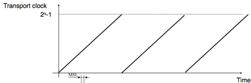
Figure 4.26: Transport clock
