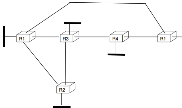
Figure 5.94: The five routers lab
