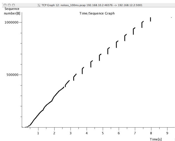
Figure 4.66: Wireshark : sequence number graph
