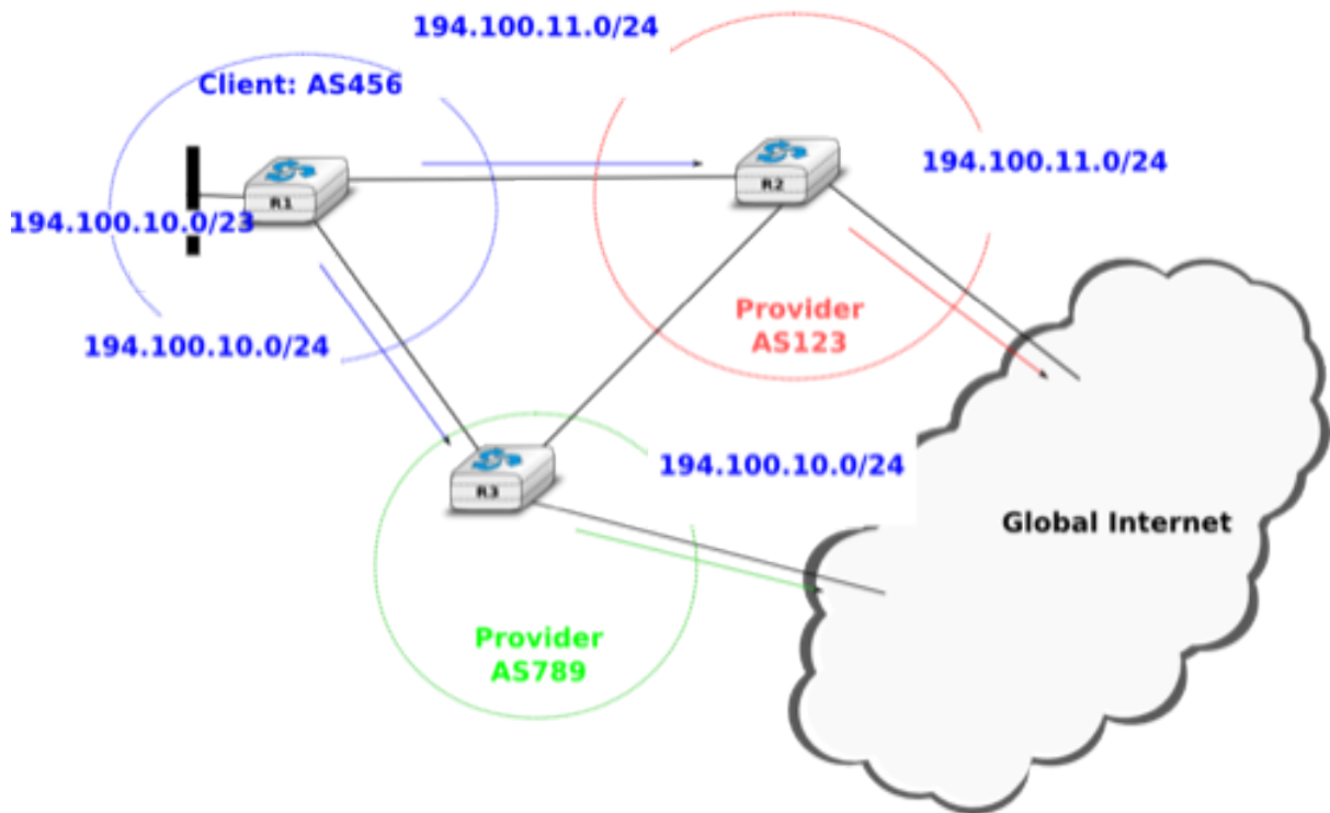
Figure 5.88: A stub connected to two providers
