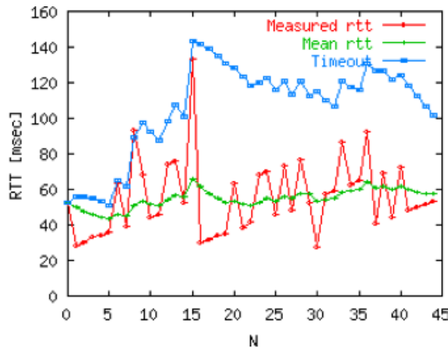
Figure 4.46: Example computation of the rto
