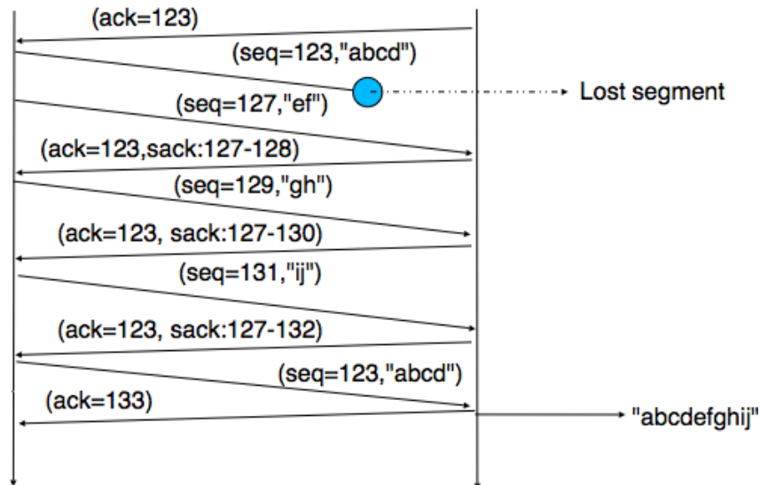
Figure 4.49: TCP selective acknowledgements
