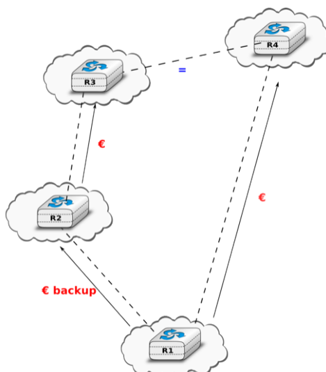
Figure 5.91: A simple internetwork with a backup link
