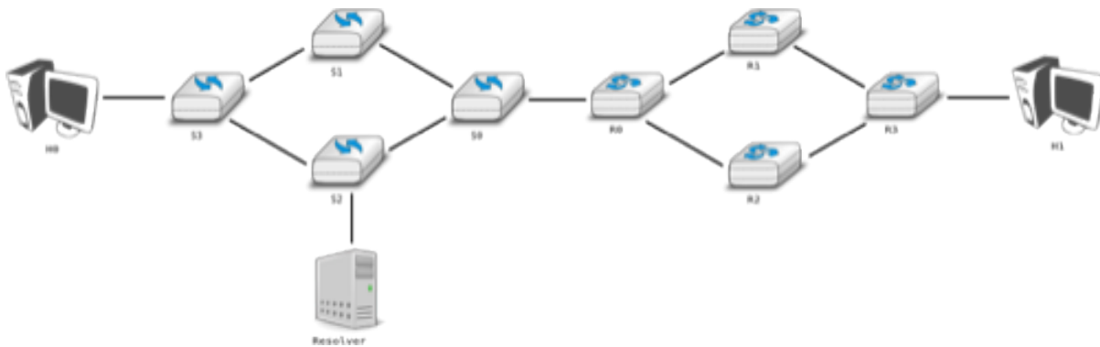
Figure 6.39: The host H0 performs a traceroute toward its peer H1 through a network composed of switches and routers.
