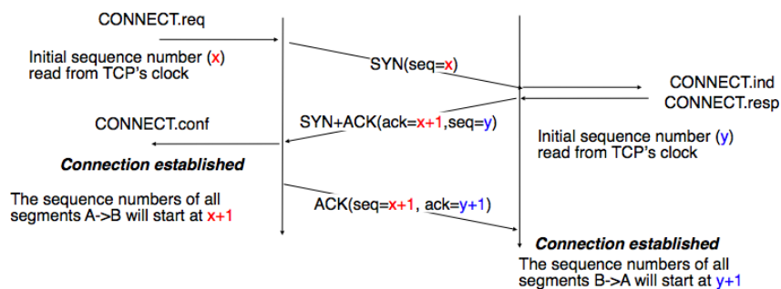
Figure 4.37: Establishment of a TCP connection
