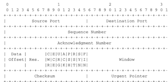
Figure 4.35: TCP header format
