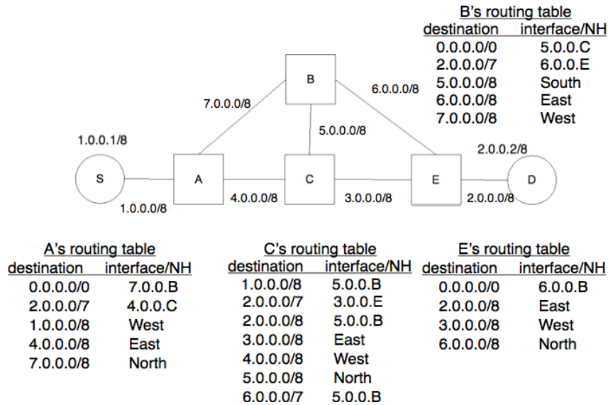
Figure 5.82: A small network
