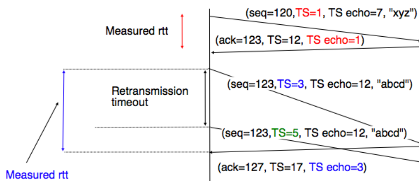
Figure 4.45: Disambiguating round-trip-time measurements with the RFC 1323 timestamp option
