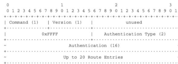
Figure 5.47: RIP message format
