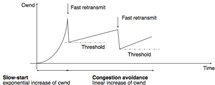
Figure 4.57: Evaluation of the TCP congestion window when the network is lightly congested
