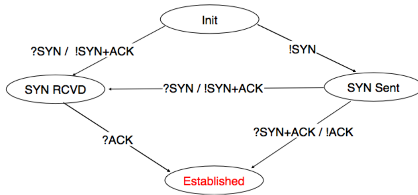
Figure 4.39: TCP FSM for connection establishment
