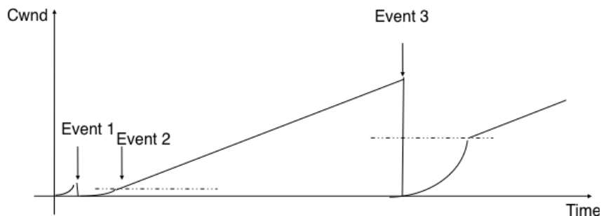
Figure 4.61: Evolution of the congestion window
