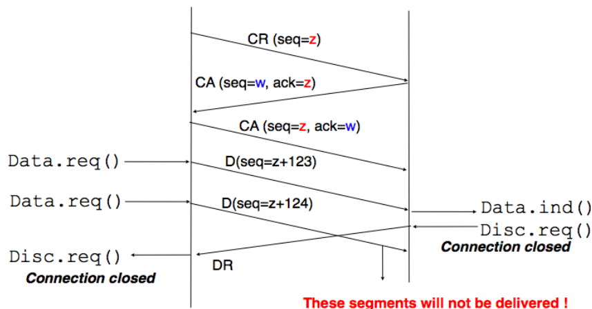
Figure 4.31: Abrupt connection release
