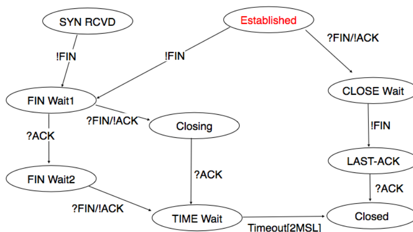
Figure 4.41: FSM for TCP connection release
