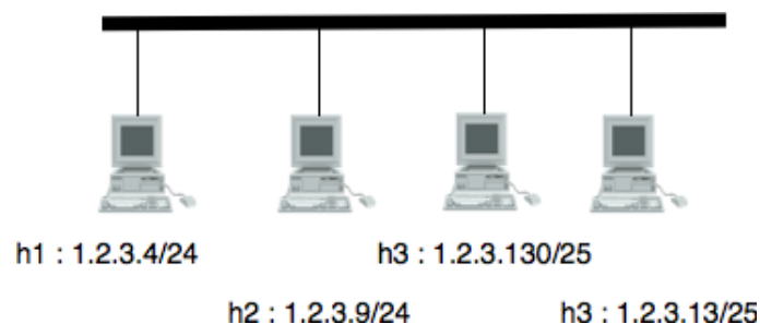
Figure 5.84: Misconfigured hosts on a subnetwork
