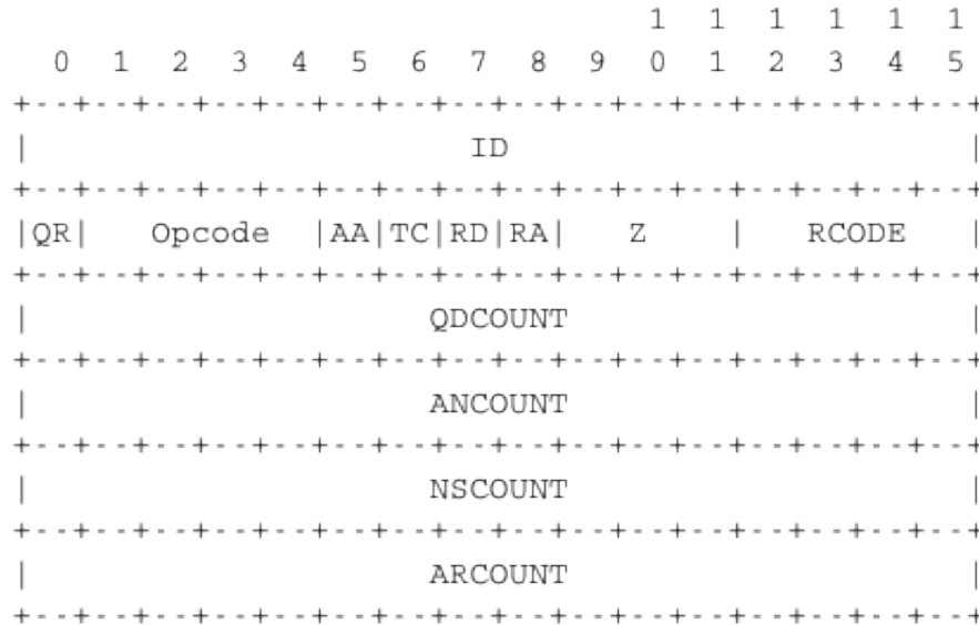
Figure 3.9: DNS header
