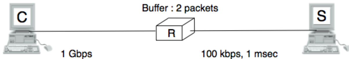
Figure 4.59: Simple network
