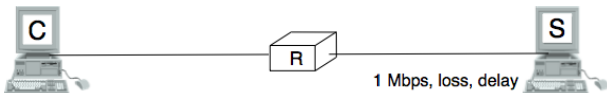
Figure 4.68: Emulated network
