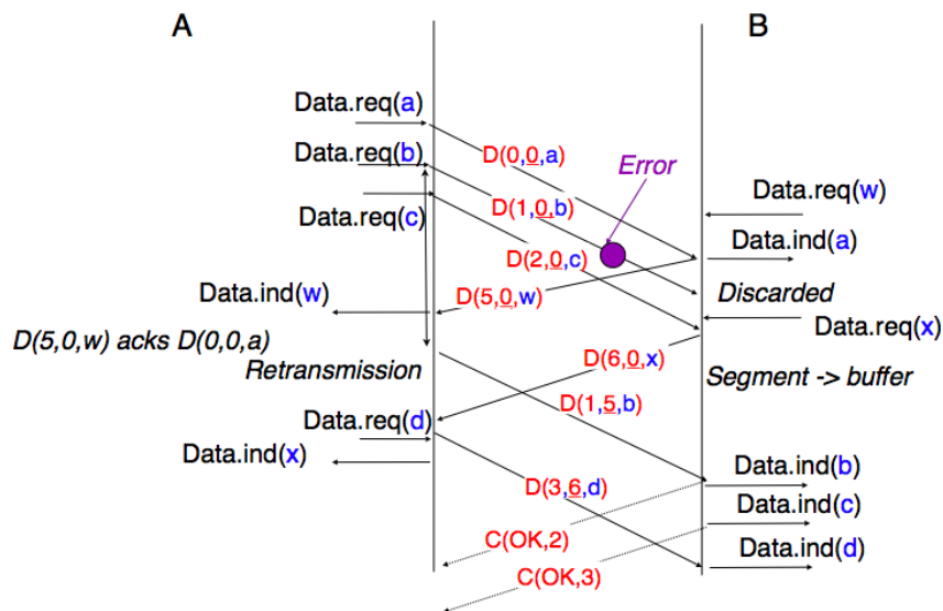
Figure 4.22: Piggybacking
