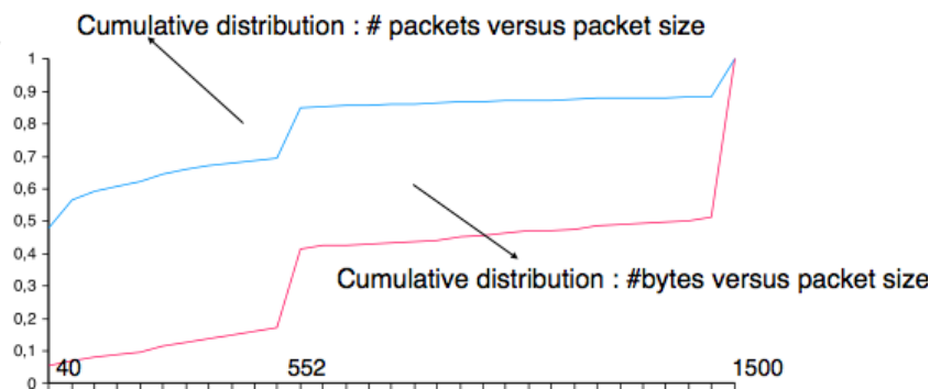
Figure 4.42: Packet size distribution in the Internet
