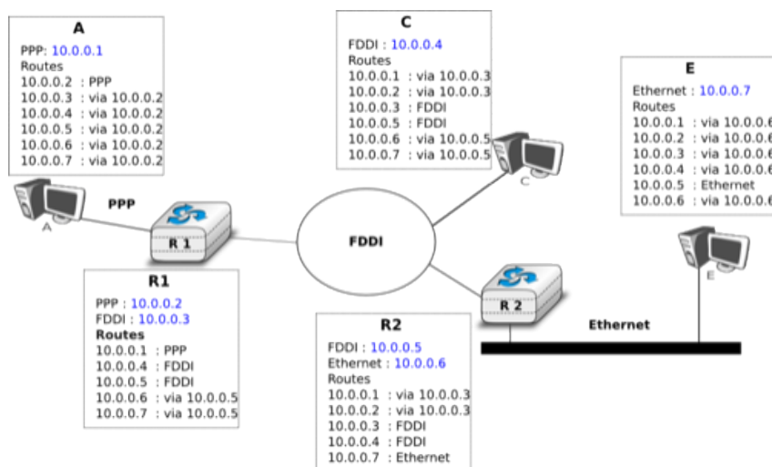
Figure 5.19: Scalability issues when using isolated IP addresses
