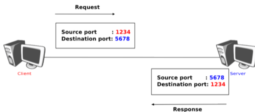
Figure 4.33: Usage of the UDP port numbers
