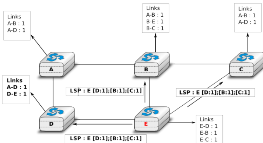
Figure 5.14: Flooding : example
