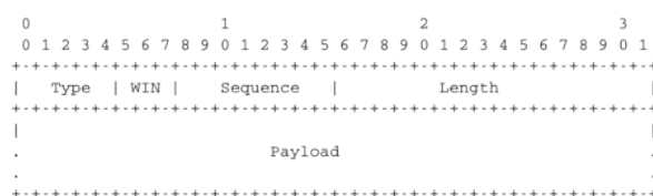
Figure 4.63: Segment format
