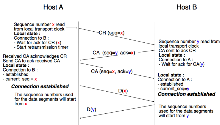
Figure 4.27: Three-way handshake
