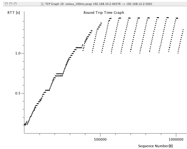
Figure 4.67: Wireshark : round-trip-time graph
