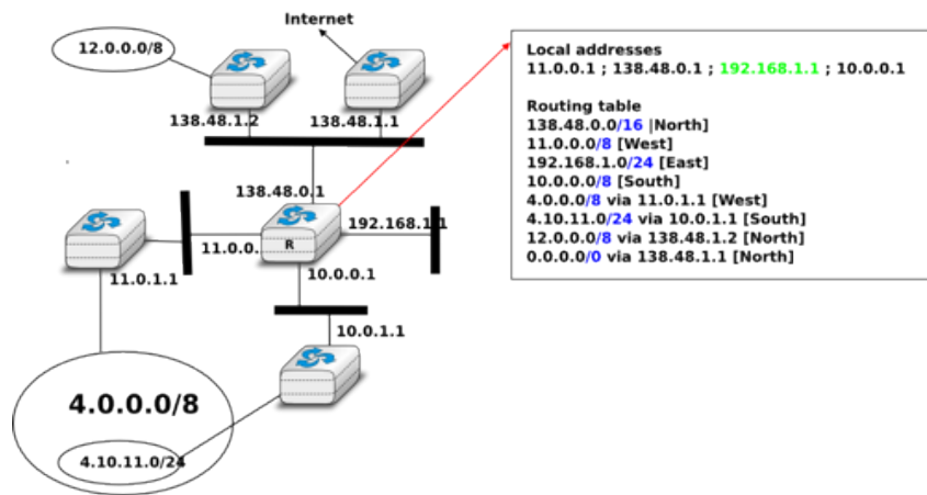
Figure 5.24: Longest prefix match example
