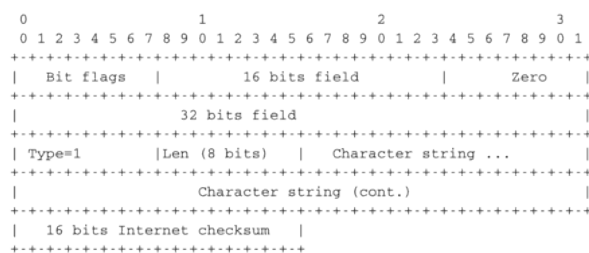
Figure 4.62: Simple SDU format
