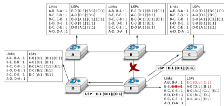
Figure 5.16: The two-way connectivity check
